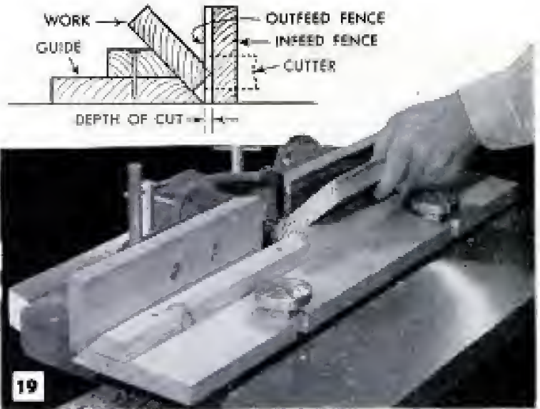
Beveling and chamfering cuts are run on shaper with a special angle guide. Adjustable shaper fence determines depth of cut
